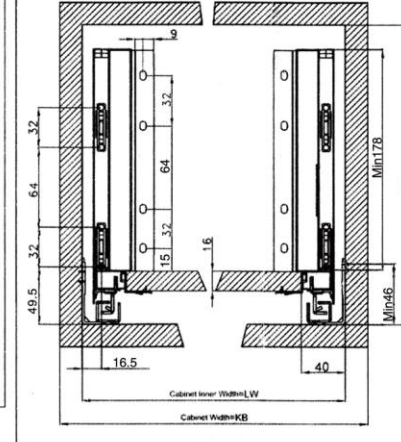
Slide installation Spec. - 907H
