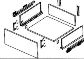
Slide installation Spec. - 907H
