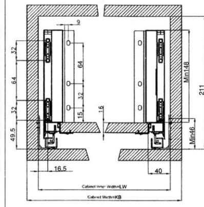
Slide installation Spec. - 907G
