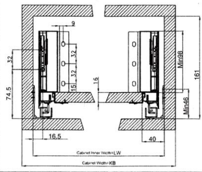
Slide installation Spec. - 907L
