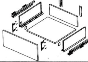
Slide installation Spec. - 907G
