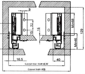
Slide installation Spec. - 907P
