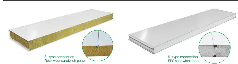
S type connection sandwich panel Width : 950/1150mm
