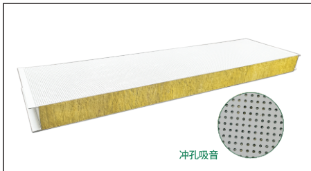
Rock wool sound absorbing panel Width : 950/1150mm
