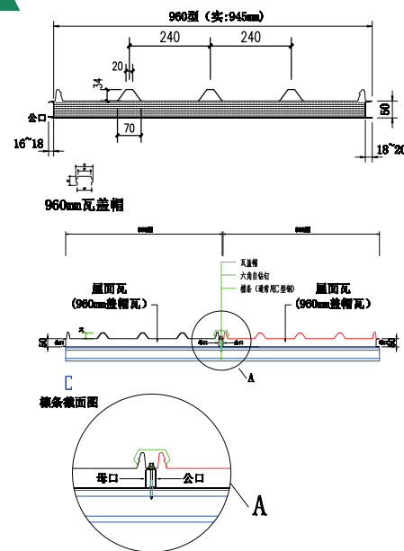
Rock wool roof sandwich panel Width : 960mm
