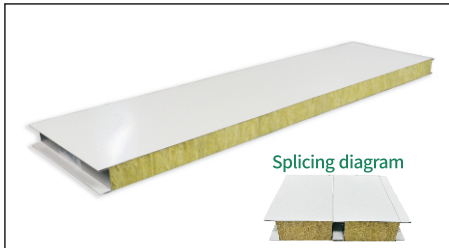
Rock wool sandwich panel Width : 950/1150mm
