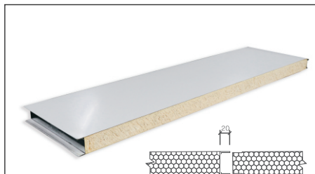
Phenolic sandwich panel Model: 950/1150mm
