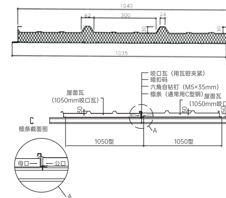
PU roof sandwich panel Width : 1050mm
