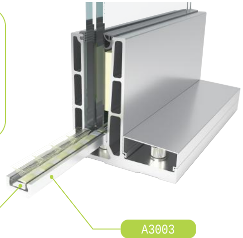
LED灯架 LED Strip Holder
