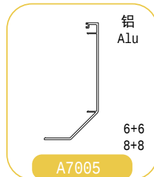
装饰盖 Decorative Cover
