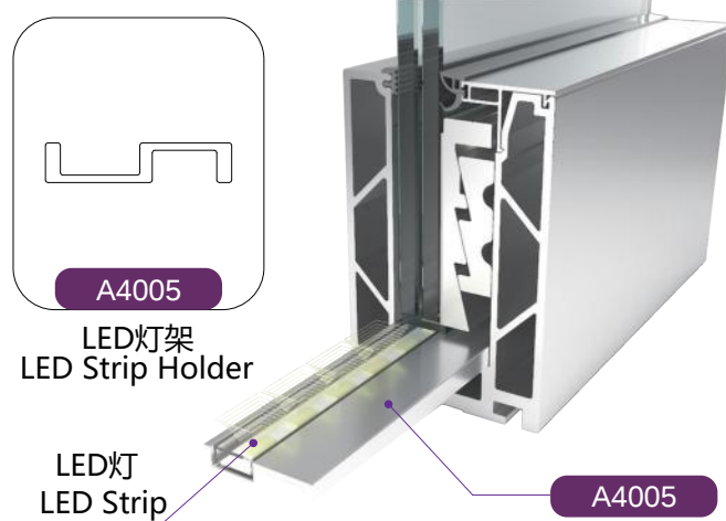
LED灯带 LED Strip
