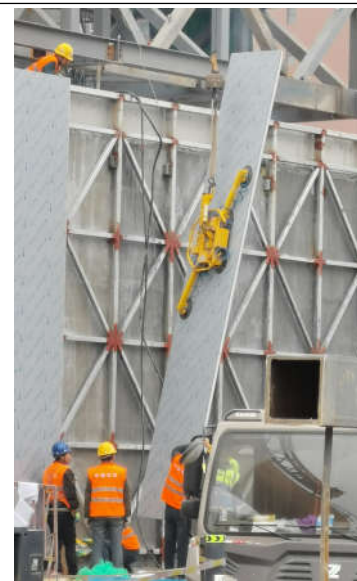
吊装板材/Lifting plate
